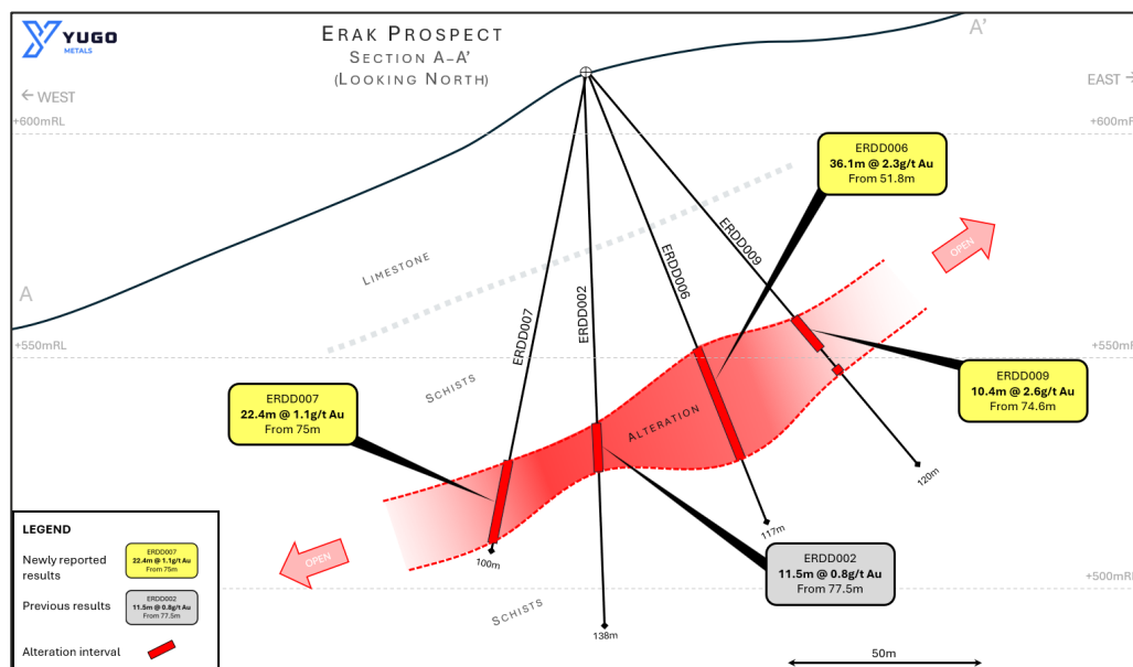
Figure 2: Erak Prospect (Golden Hills Project), drilling cross-section A-A'
