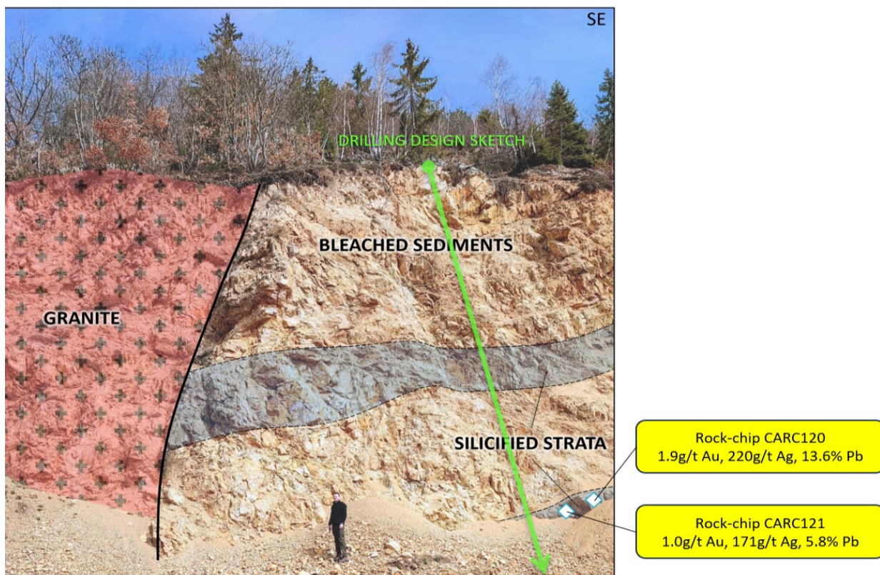
Figure 4: Monte Project, Majdan Au-Ag-Pb Prospect, photo of cliff profile
