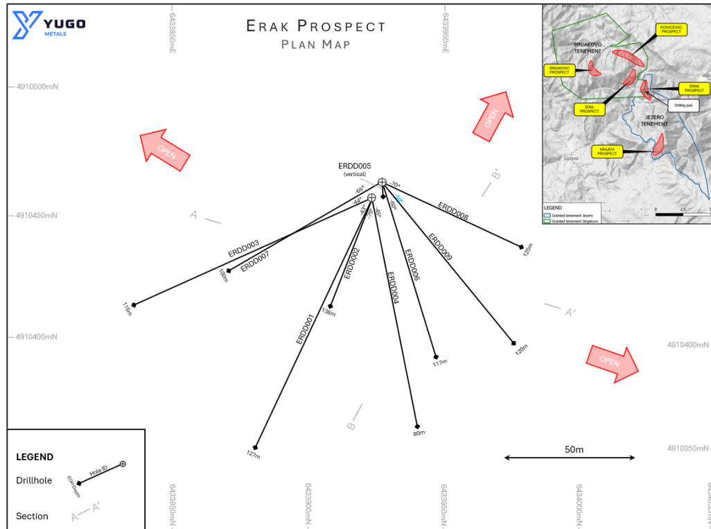
Figure 1 Erak Prospect (Golden Hills Project), plan map showing drilling program
