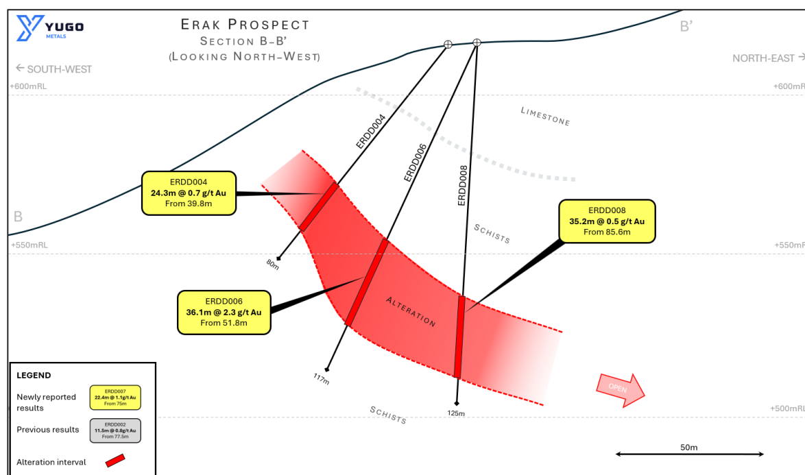
Figure 3: Erak Prospect (Golden Hills Project), drilling cross-section B-B'
