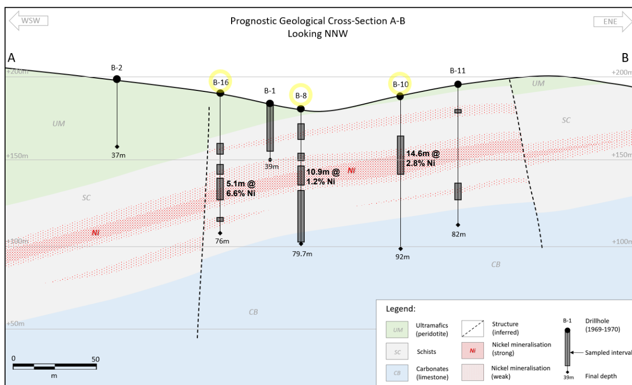
Figure 6: Petrovo cross-section showing historical drill holes with interpreted geology
