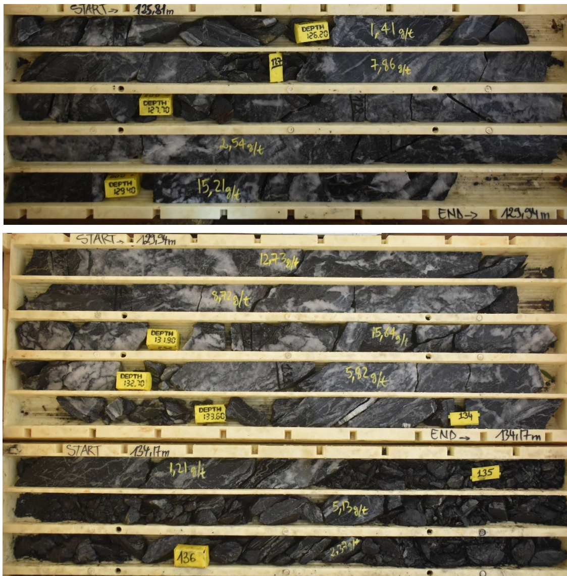
Photo One | Adiopan (ADIDD0012) Drill Core 126m-136m
