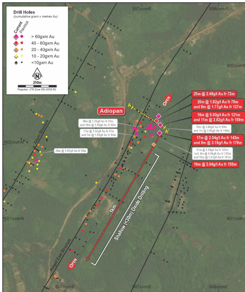
Figure Three | Adiopan Drill Plan
