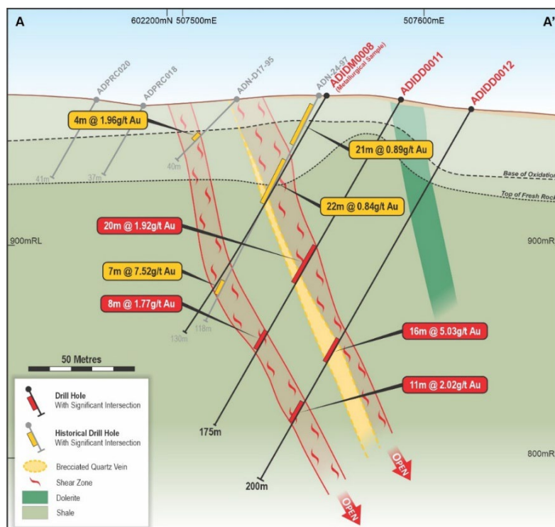
Figure Four | Adiopan Cross Section
