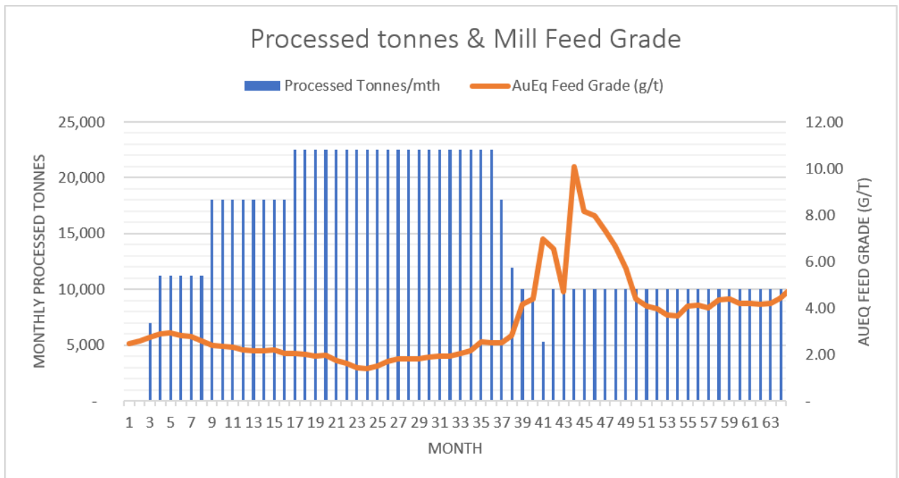
Figure 8: Mt Moss Mill processing schedule.
