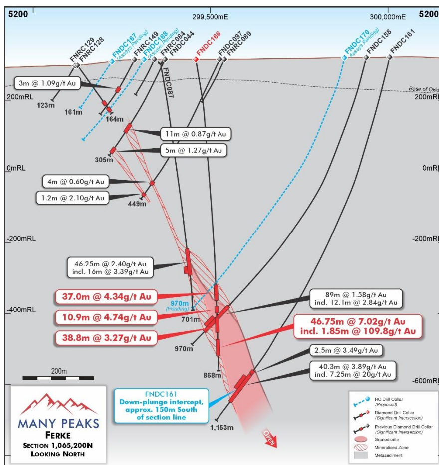
Figure 1 | Cross Section 1,065,200N (refer to Figure 4 for location in plan view) with interpreted geometry of mineralised zone and location of significant intercepts in drilling (reported results annotated in red)
