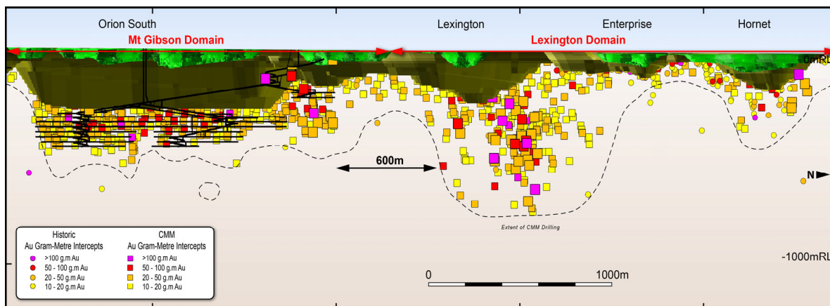
Figure 1 – Long section along the Orion South-Hornet trend. Large squares denote significant assay results received since the previous update.
