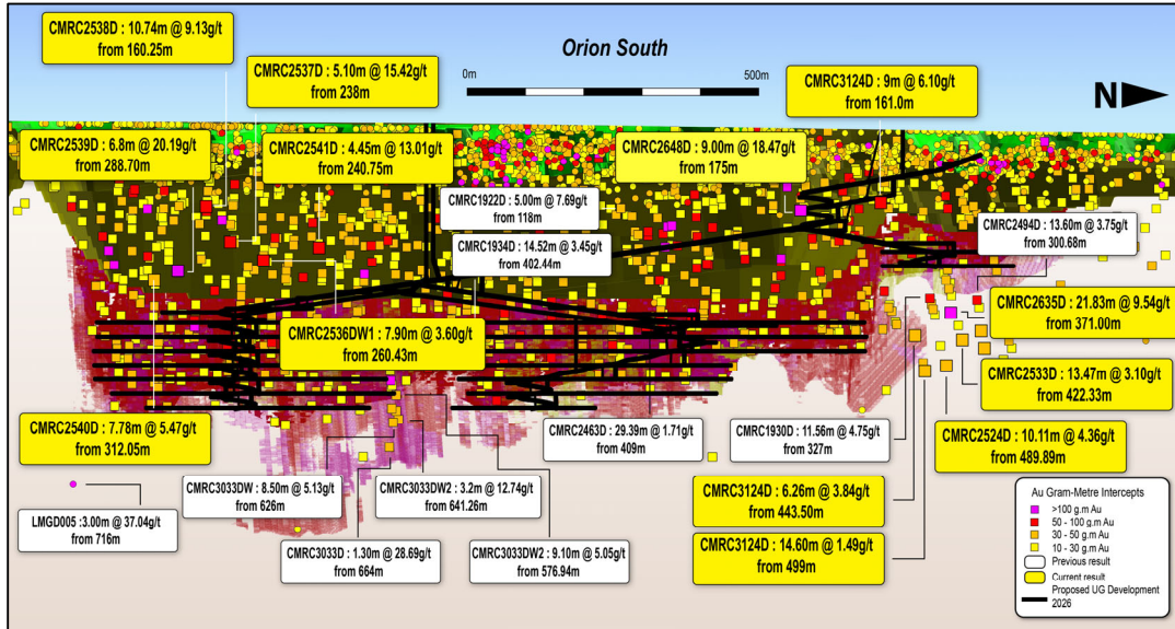
Figure 5 – Orion South long section looking west, highlighting over 1,600m of prospective strike defined by recent intersections exceeding 25 gram-metres Au. Significant high-grade mineralisation extends beyond the current Ore Reserve outline (A$2,200/oz) and Mineral Resource optimisation outline (A$2,800/oz).
