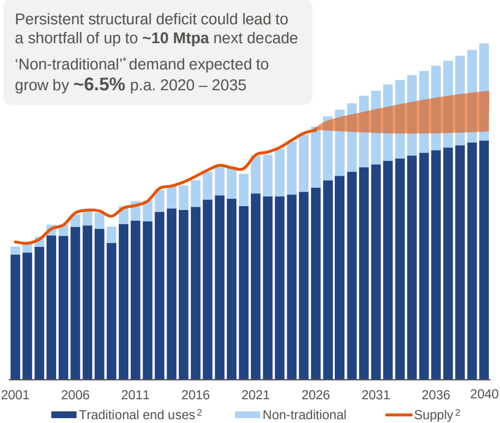
Copper demand and supply, 2001 – 2040 (Mt)
