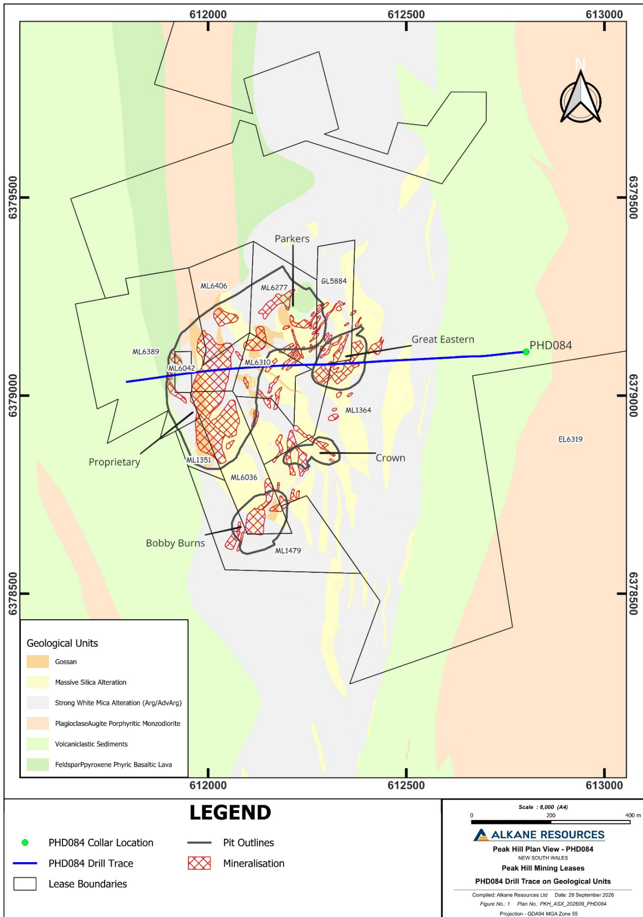
Figure 5 – Local geology and mineralisation of the Peak Hill Gold Mine with drill hole trace PHD084.
