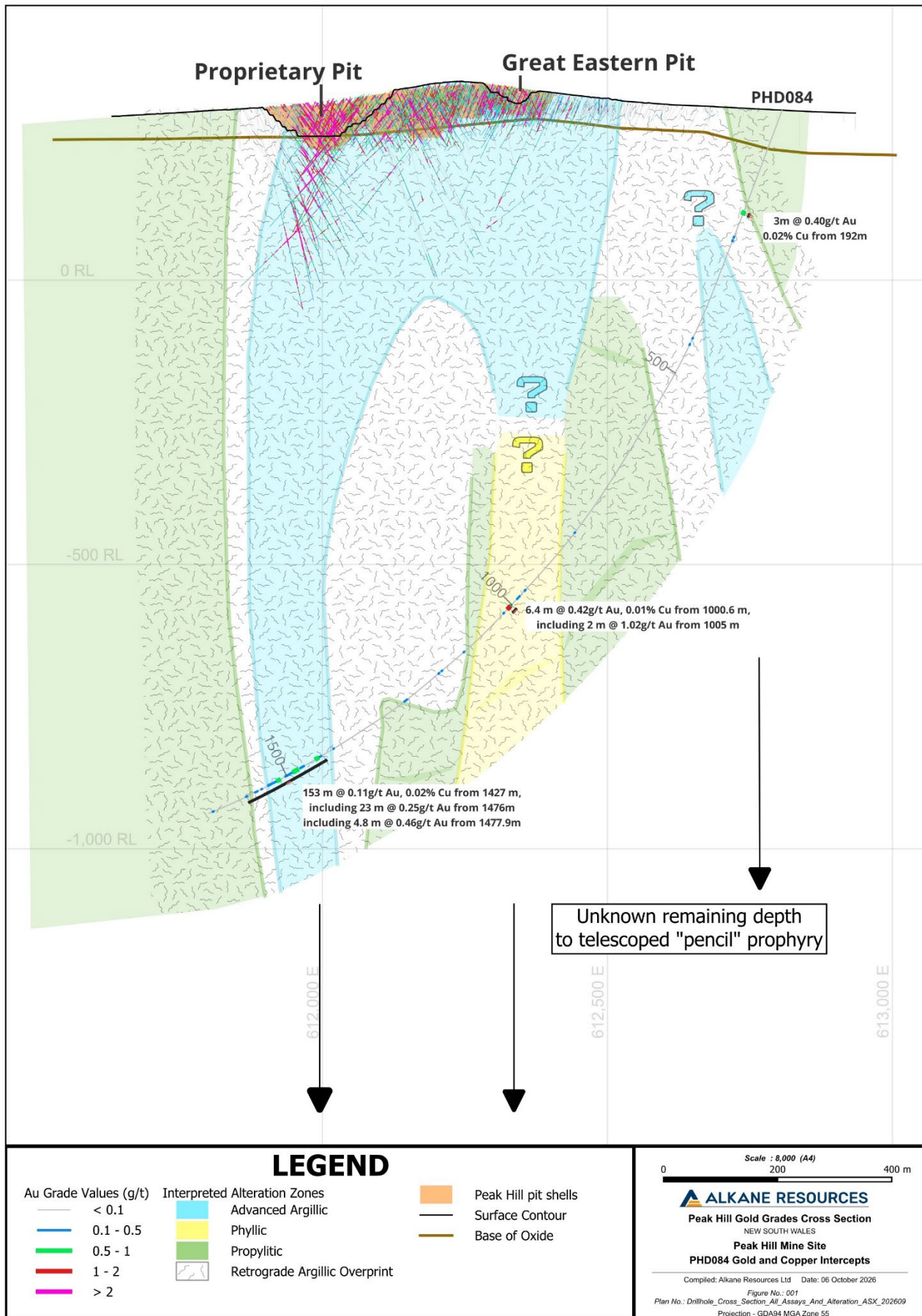
Figure 6 - Section of general alteration assemblages informed by short wave infrared spectral scanning.
