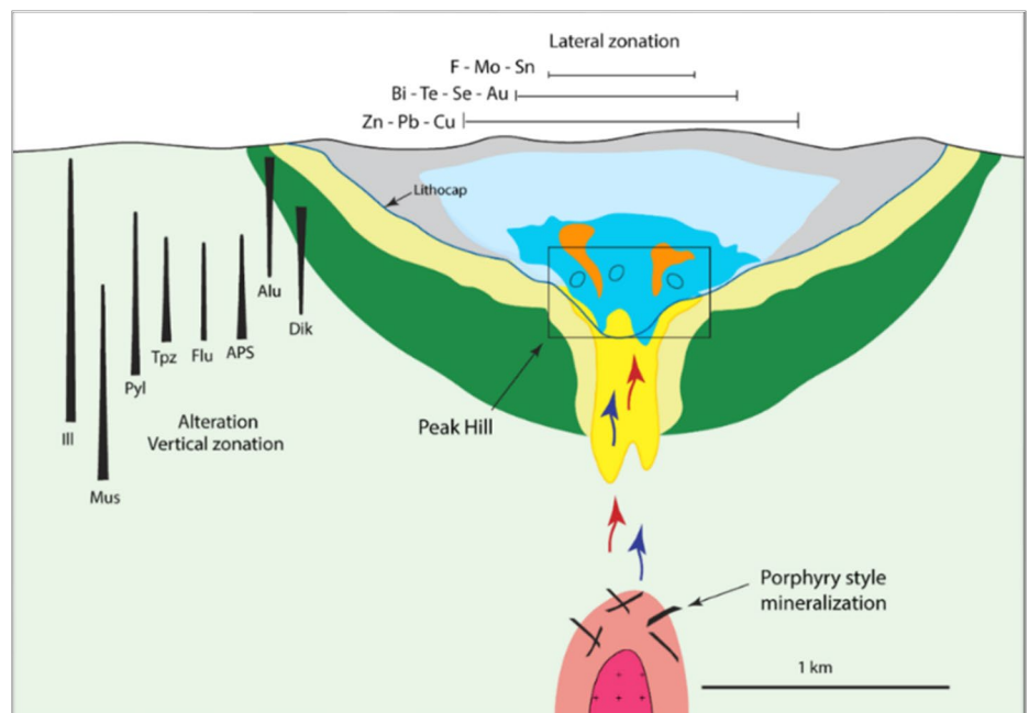
Figure 1. Schematic model of Peak Hill in the porphyry-epithermal environment.
