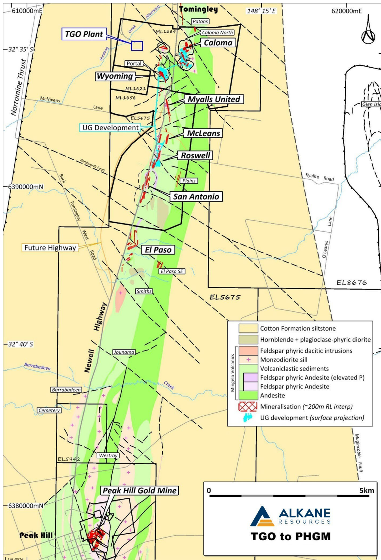
Figure 2. Basement geology from Peak Hill Gold Mine to Tomingley Gold Operations.
