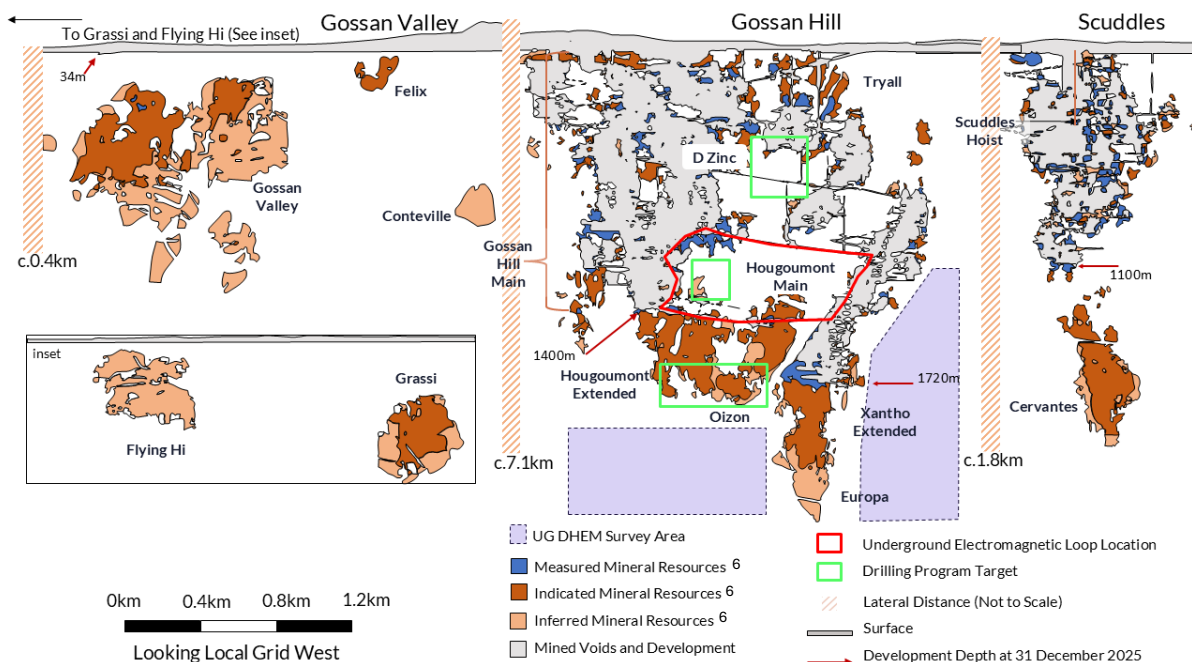
Figure 6: Golden Grove long-section highlighting drill program target areas, EMTL location and survey areas
