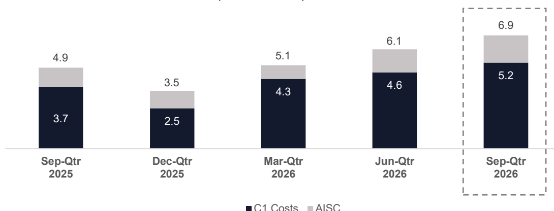
Figure 3: Golden Grove C1 Costs 2 and AISC 5 (US$/lb Cu sold)
