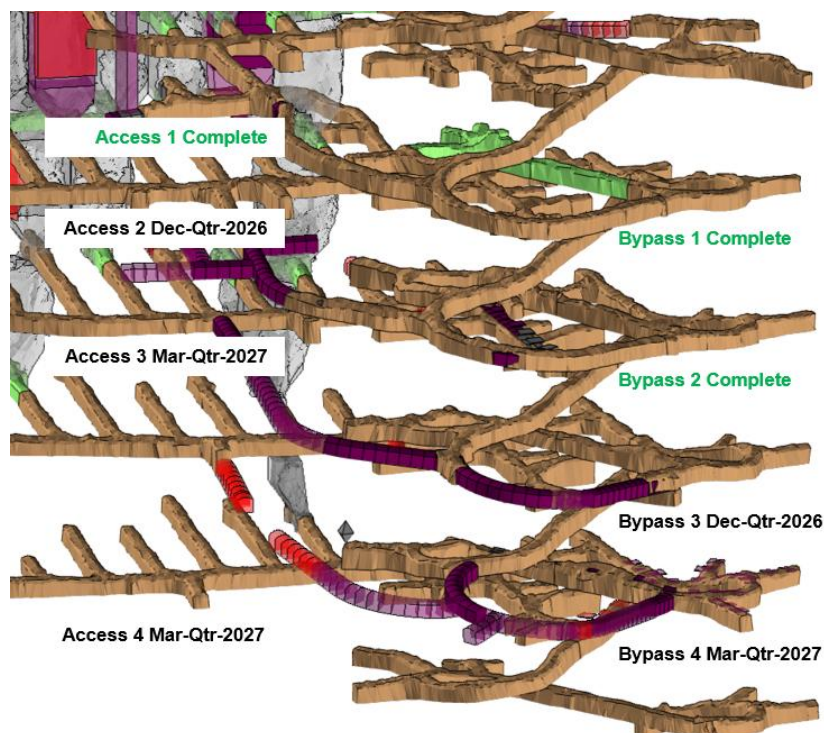
Figure 4: Xantho Extended underground development, October 2026
